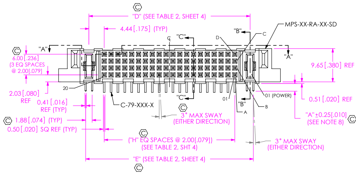
FIG 1 MPSC-01-80-01-01-01-X-RA-SD SHOWN
