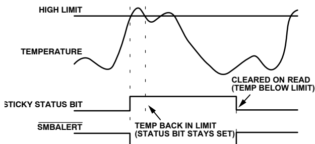
Figure 38. \overline{\text{ALERT}} and Status Bit Behavior
