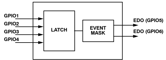
Figure 84. EDO Circuit
