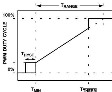
Figure 64. T_{HYST} Value Applies to Fan On/Off Hysteresis
