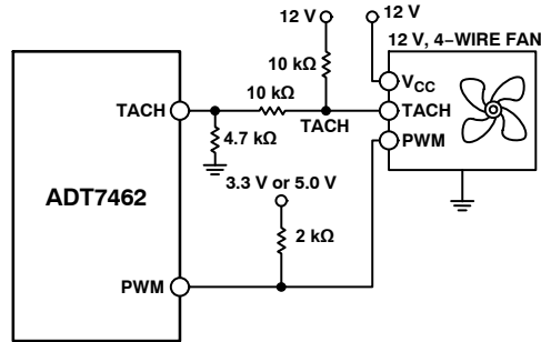
Figure 41. Driving a 4-Wire Fan
