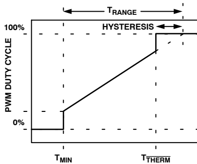
Figure 63. How T_{THERM} Relates to Automatic Fan Control
