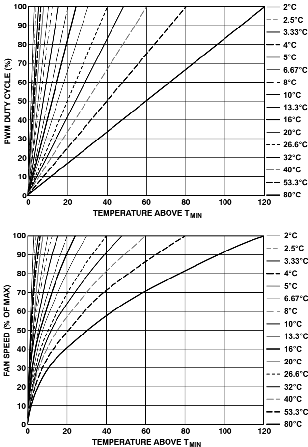
Figure 60. T RANGE vs. Actual Fan Speed Profile
