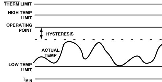
Figure 70. Temperature Between the Operating Point and the Low Temperature Limit
