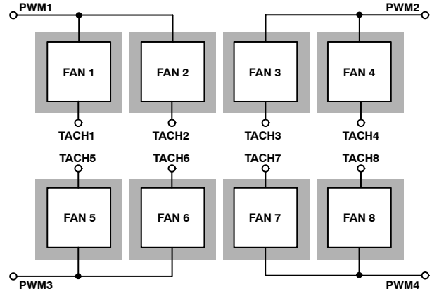
Figure 48. Synchronizing Fan PWM Output and TACH Inputs
