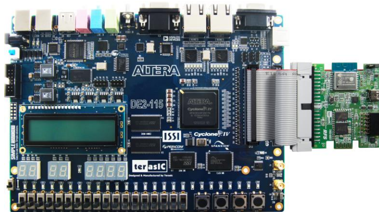
Figure 1-9 Connect the RFS to DE2-115
