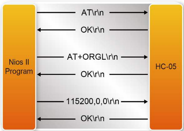
Figure 4-14 Handshake Chart
