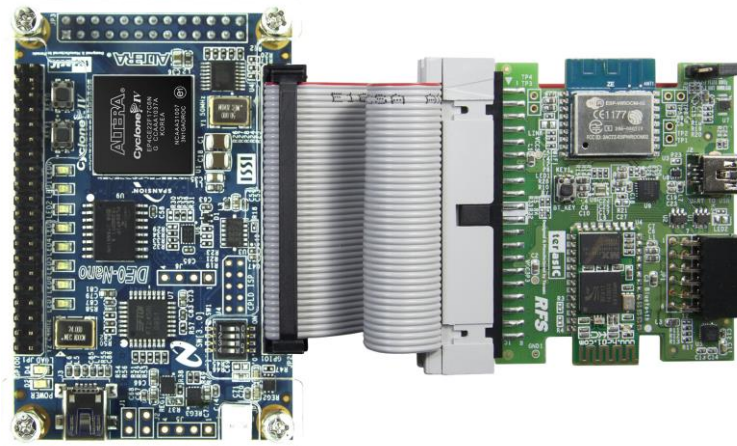
Figure 1-6 Connect the RFS to DE0-Nano
