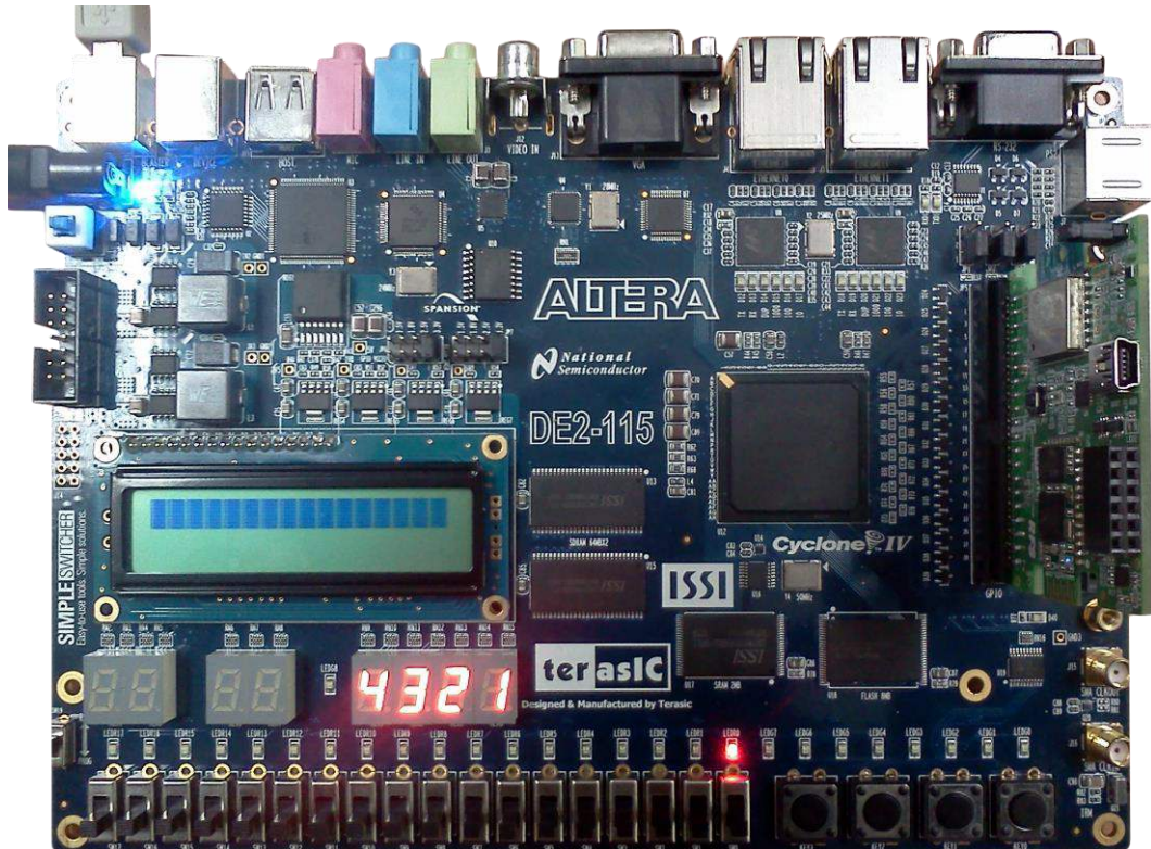
Figure 3-15 Sensor RTL Code Demo setup on DE2-115
