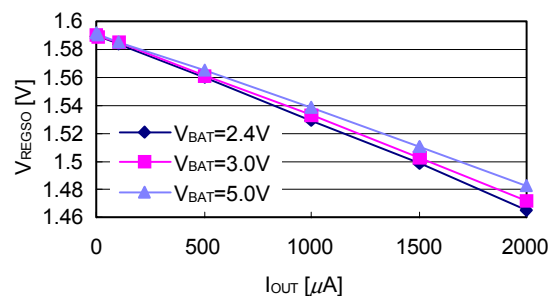
Figure 15 V REGSO Characteristics
