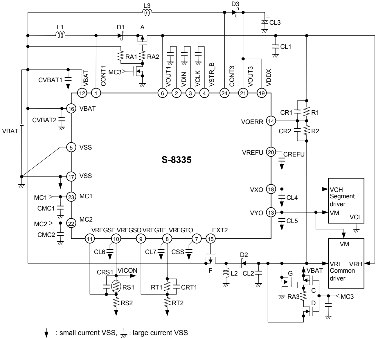
Figure 21 Application Circuit Example
