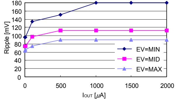
DC/DC P part output ripple voltage (V BAT = 5.0 V, reference value)
