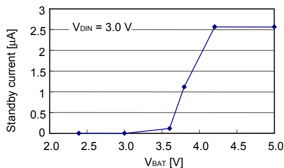
Figure 11 Standby Mode Current Characteristics
