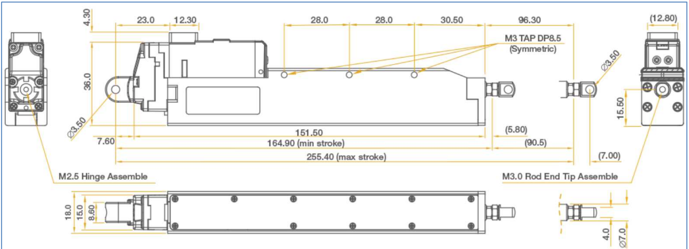
Figure 4.Dimension
