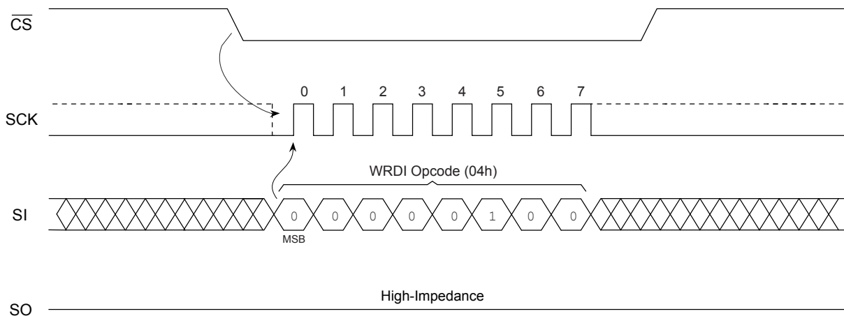
Figure 6-3. \overline{\text{WRDI}} Timing
