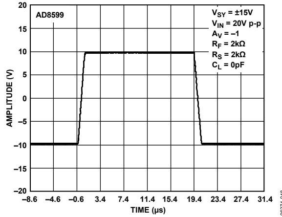
Figure 50. Large Signal Response
