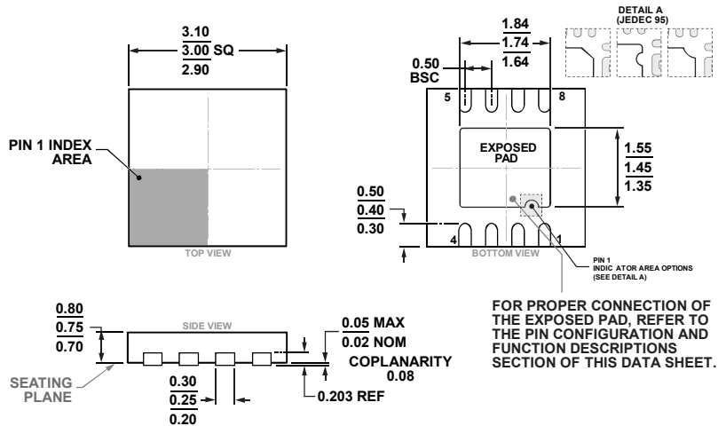
Figure 61. 8-Lead Lead Frame Chip Scale Package [LFCSP] 3 mm x 3 mm Body and 0.75 mm Package Height (CP-8-13)
