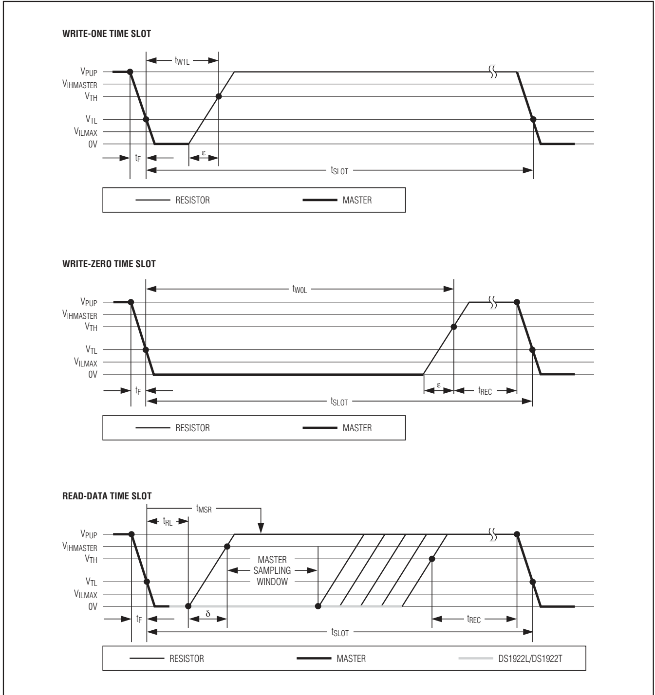
Figure 13. Read/Write Timing Diagrams
