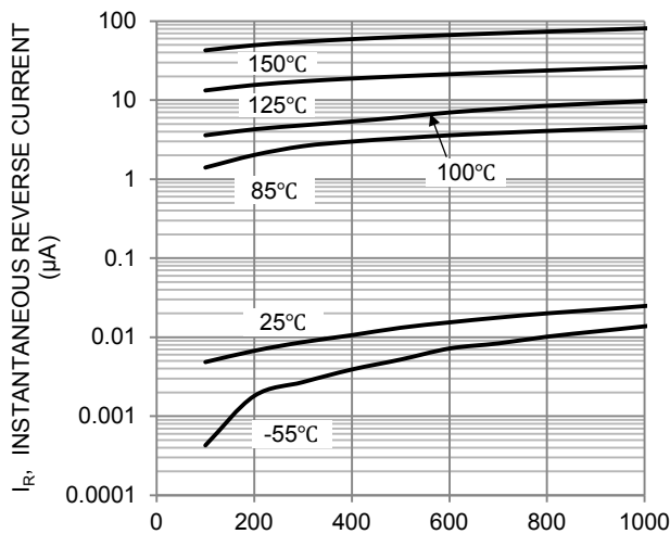
V_R , INSTANTANEOUS REVERSE VOLTAGE (V) Figure 5. Typical Reverse Characteristics (Per Leg)
