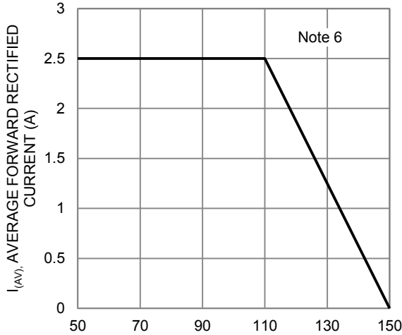
T_C , CASE TEMPERATURE ( ^{\circ}C ) Figure 1. Output Current Derating Curve
