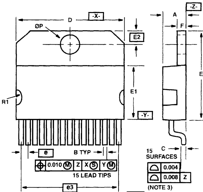
Z15.05B 15 LEAD PLASTIC SINGLE-IN-LINE PACKAGE SURFACE MOUNT "GULLWING" LEAD FORM
