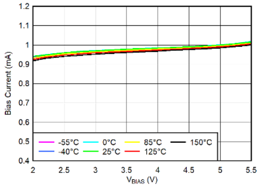
Figure 5-34. BIAS Pin Current vs V BIAS and Temperature (T J )
