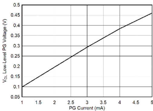
Figure 5-36. Low-Level PG Voltage vs Current
