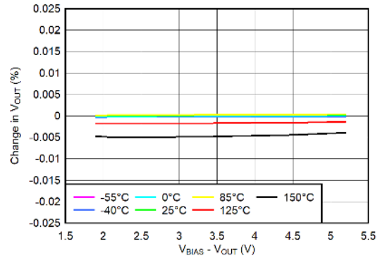
Figure 5-23. V_{BIAS} Line Regulation
