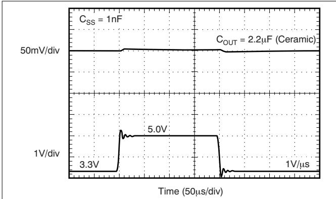
Figure 5-17. V_{BIAS} Line Transient
