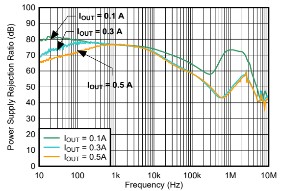
Figure 5-31. V_{IN} PSRR vs Frequency
