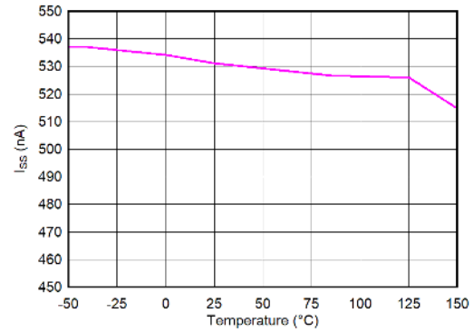
Figure 5-35. Soft-Start Charging Current (I SS ) vs Temperature (T J )
