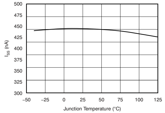
Figure 5-14. Soft-Start Charging Current (I SS ) vs Temperature (T J )
