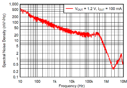
Figure 5-32. Noise Spectral Density
