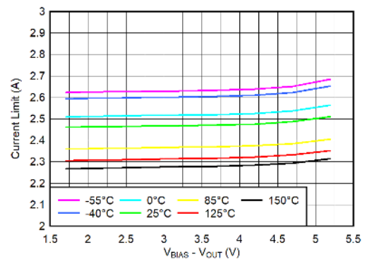
Figure 5-37. Current Limit vs (V BIAS – V OUT )
