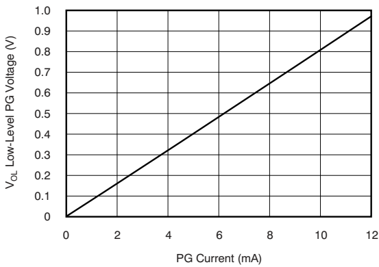
Figure 5-15. Low-Level PG Voltage vs Current
