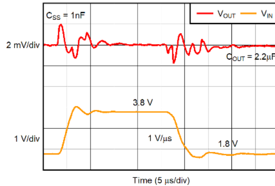
Figure 5-39. V_{IN} Line Transient
