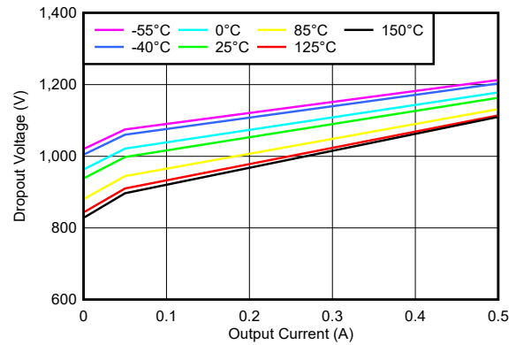
Figure 5-29. V_{BIAS} Dropout Voltage vs I_{OUT} and Temperature ( T_J )
