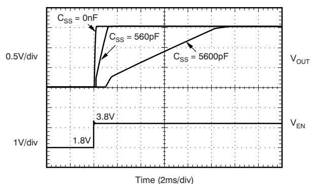
Turn-On Response
