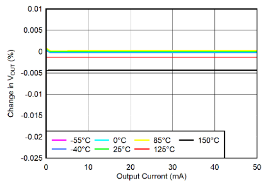
Figure 5-25. Load Regulation at Light Load
