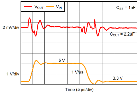
Figure 5-38. V_{BIAS} Line Transient
