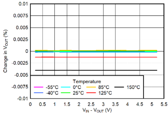
Figure 5-22. V_{IN} Line Regulation
