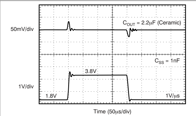
Figure 5-18. V_{IN} Line Transient
