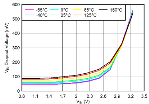
Figure 5-27. V_{IN} Dropout Voltage vs V_{IN} and Temperature ( T_J ) for I_{OUT} = 500 \text{ mA}
