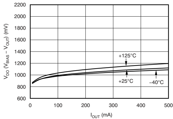
Figure 5-7. V_{BIAS} Dropout Voltage vs I_{OUT} and Temperature ( T_J )
