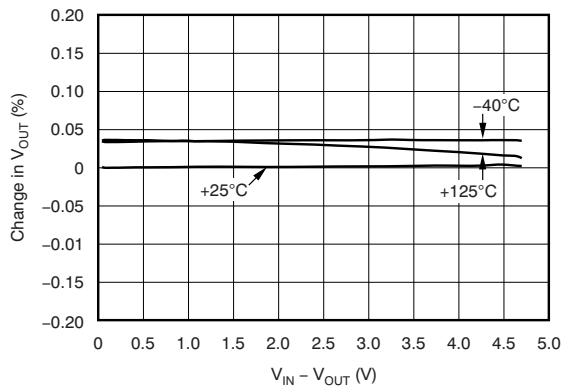
Figure 5-1. V IN Line Regulation
