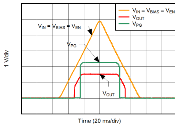
Figure 5-42. Power-Up and Power-Down
