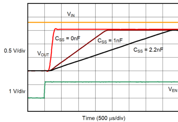
Figure 5-41. Turn-On Response
