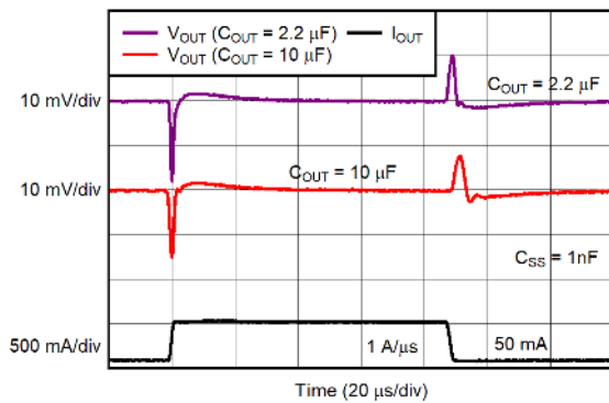
Figure 5-40. Output Load Transient Response
