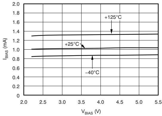
Figure 5-13. BIAS Pin Current vs V BIAS and Temperature (T J )
