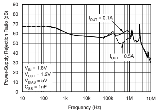
Figure 5-8. V_{BIAS} PSRR vs Frequency
