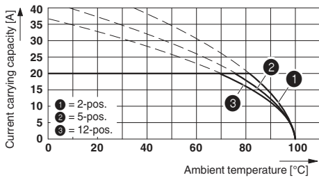
Derating curve for: PC 4/12-ST-7,62 with PC 4/1-G-7,62
