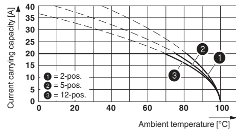
Derating curve for: PC 4/12-ST-7,62 with PCV 4/1-G-7,62
