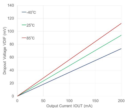
6) Dropout Voltage vs. Output Current ( C_{IN} = \text{Ceramic } 1.0\text{ }\mu\text{F}, C_{OUT} = \text{Ceramic } 1.0\text{ }\mu\text{F} )
