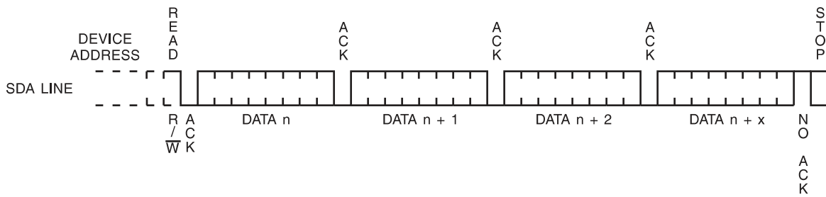
Figure 10-6. Sequential Read
