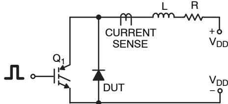
Figure 10. Avalanche Energy Test Circuit
