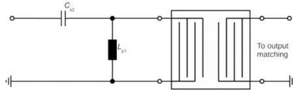
Figure 13: series C - shunt L matching.
