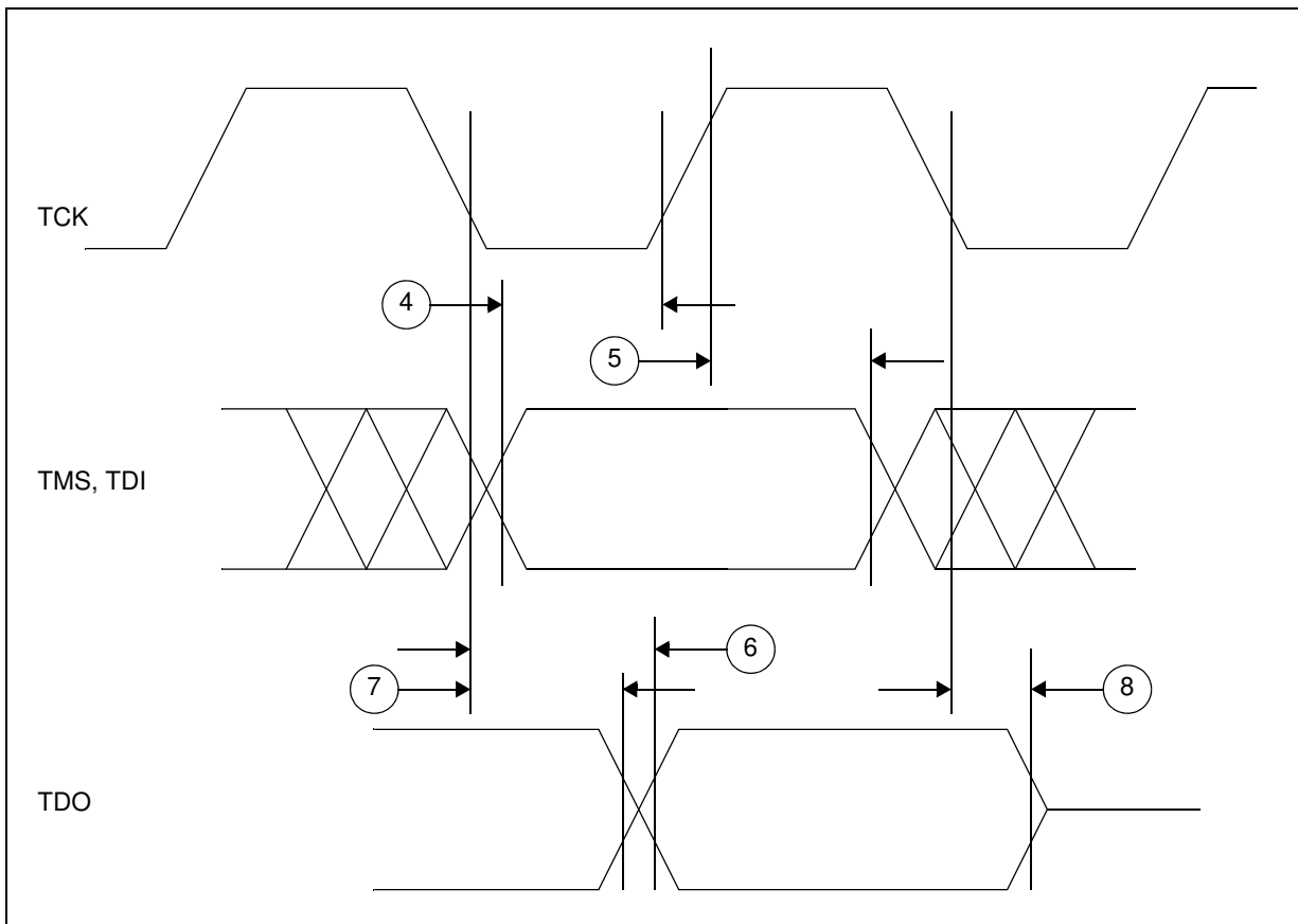
Figure 13. JTAG test access port timing
