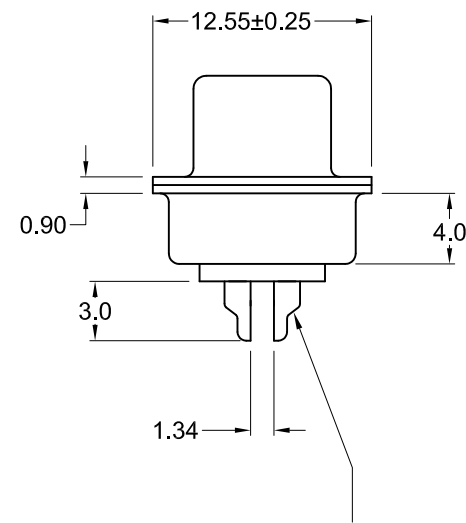
Solder Cups
