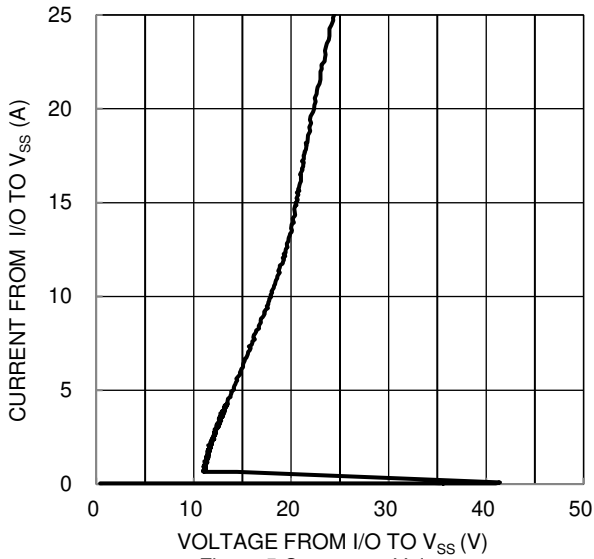
Figure 5 Current vs. Voltage
