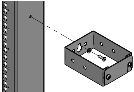
CENTER REAR HOLE MOUNTING
