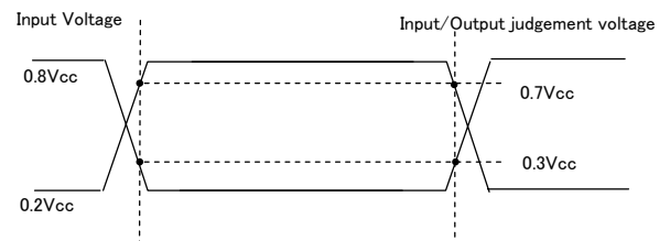
Figure 1. Input/Output judgement voltage
