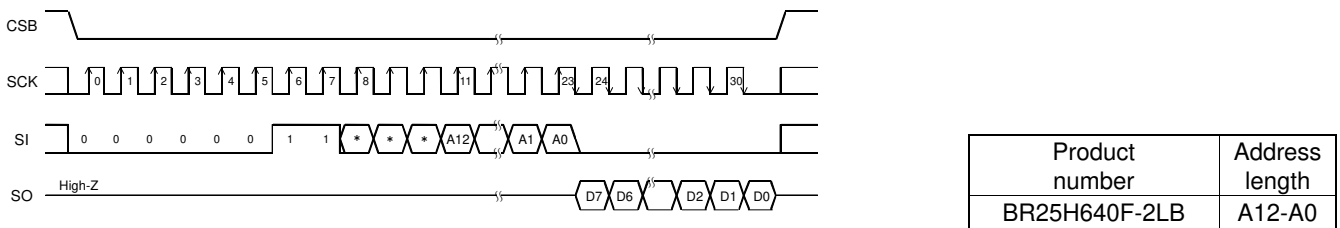
Figure 37. Read command
