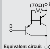
Equivalent circuit
