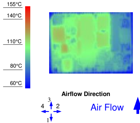
Figure 8. Thermal Image for Airflow Direction 3 (5.8A output, 55°C ambient, 200 LFM, typical Vin, open frame, unit soldered onto a fixture board)
