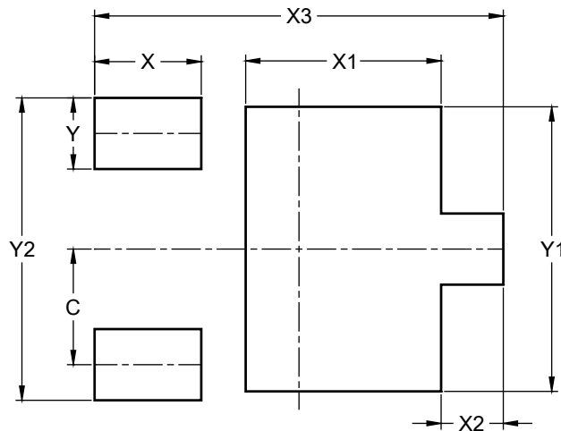
U-DFN2020-3 (Type C)
