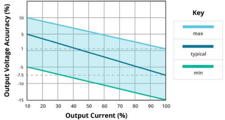
OUTPUT REGULATION CURVE 5 Vdc input / 3.3 Vdc output (nominal input)
