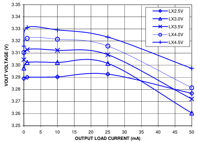
Figure 8 – LX1882-33 Output Voltage vs. Load Current; T_A = 25^\circ\text{C} , C_1 = 0.22\mu\text{F} , C_2, C_3, C_4 = 4.7\mu\text{F} , C_{\text{FILT}} = 0.1\mu\text{F}
