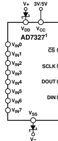
1 ADDITIONAL PINS OMITTED FOR CLARITY. 05-001-056
