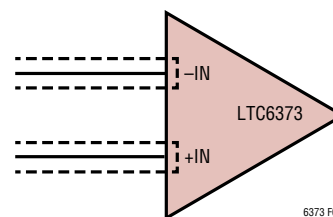
Figure 4. Guard Rings Can Be Used to Minimize Leakage into the Input Pins
