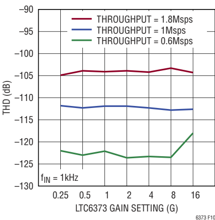
Figure 10. THD for LTC6373 Driving AD4020
