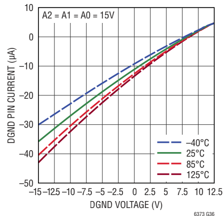
DGND Pin Current vs DGND Pin Voltage
