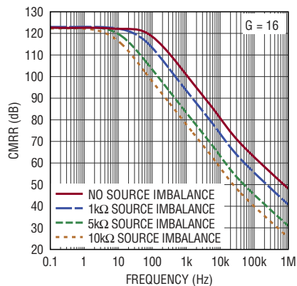
CMRR vs Frequency With Source Imbalance
