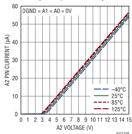
A2 Digital Input Pin Current vs A2 Digital Input Pin Voltage
