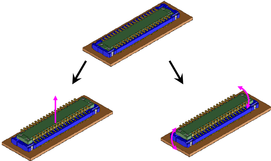
嵌合軸に沿って平行に抜く Releasing the plug paralleled to the mated axis
