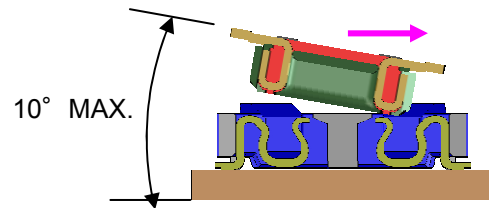
長手方向 "a" Direction (lengthways)
