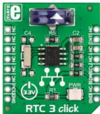
RTC 3 click
