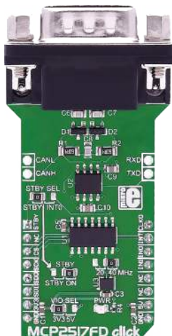
MCP2517FD click
