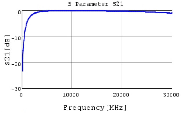
GJM0335C1E1R1CB01 S21 DCOV, 25degC
