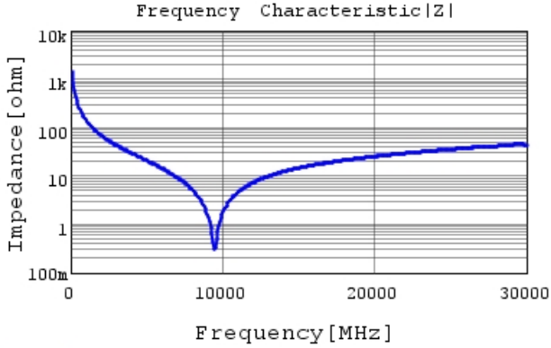
GJM0335C1E1R1CB01 |Z| DCOV,25degC
