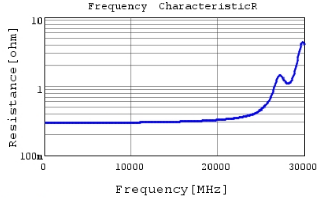
GJM0335C1E1R1CB01 R DCOV,25degC
