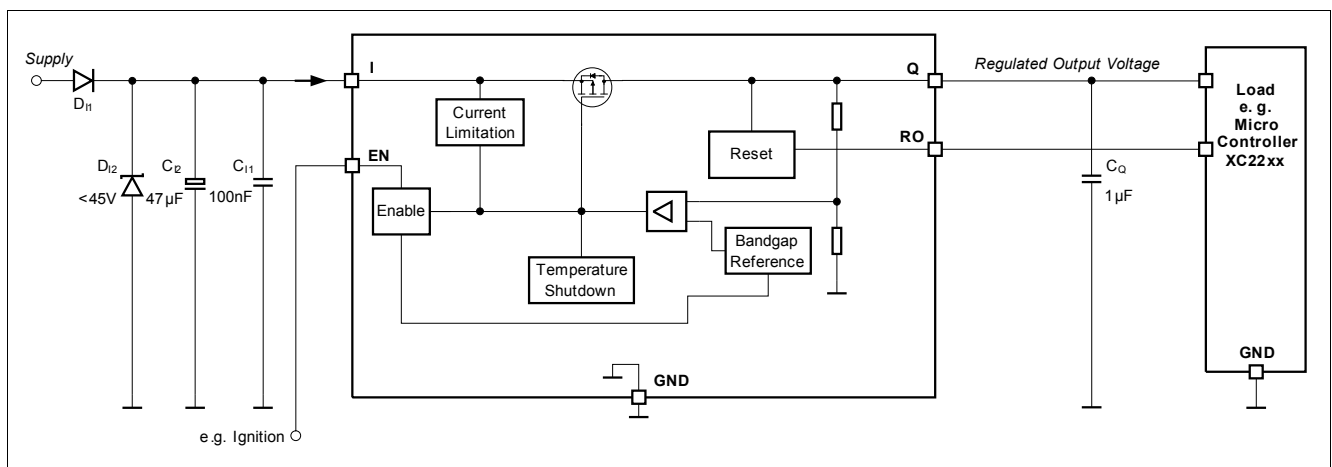
Figure 8 Application Diagram
