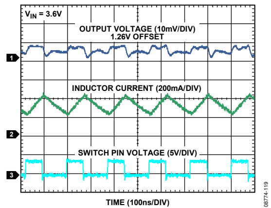
Figure 19. Standard Operation
