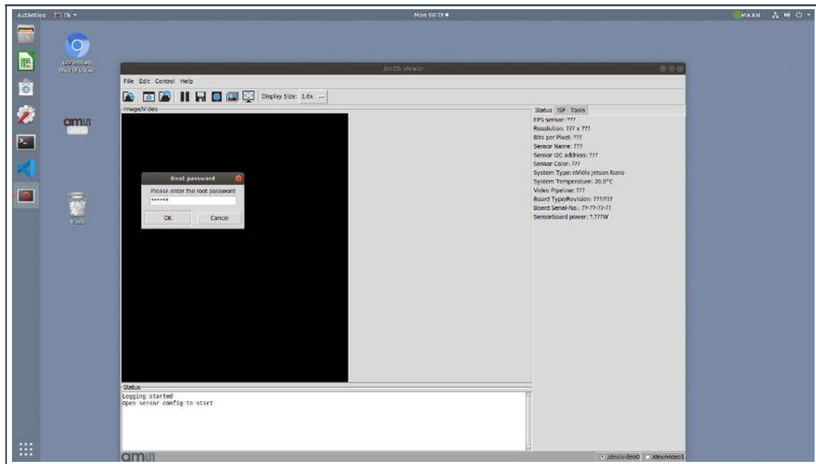
Figure 6: JetCis Viewer
