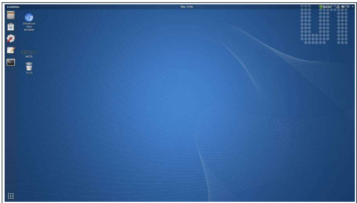
Figure 5: Desktop/Main Screen
