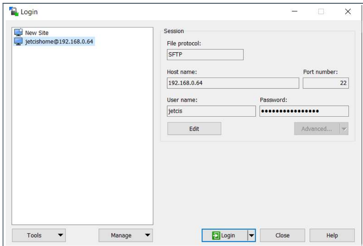
Figure 17: WinSCP
