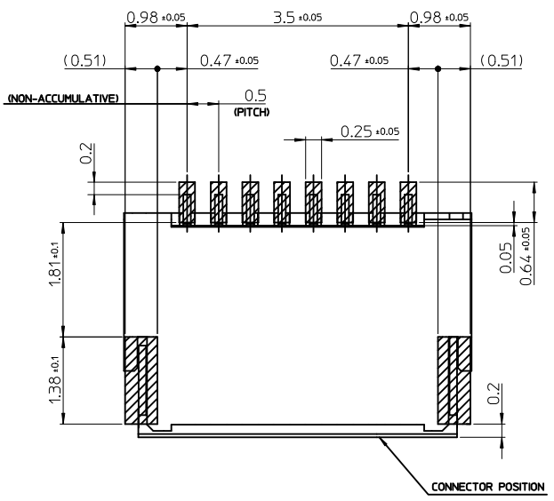
RECOMMENDED P.C.BOARD PATTERN DIMENSION(REF)
