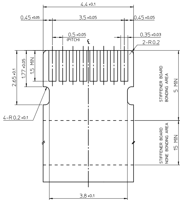
APPLICABLE FPC RECOMMENDED DIMENSION FPC THICKNESS :0.3±0.03
