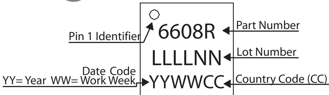
Figure 18: Branding Specification - M45 Package
