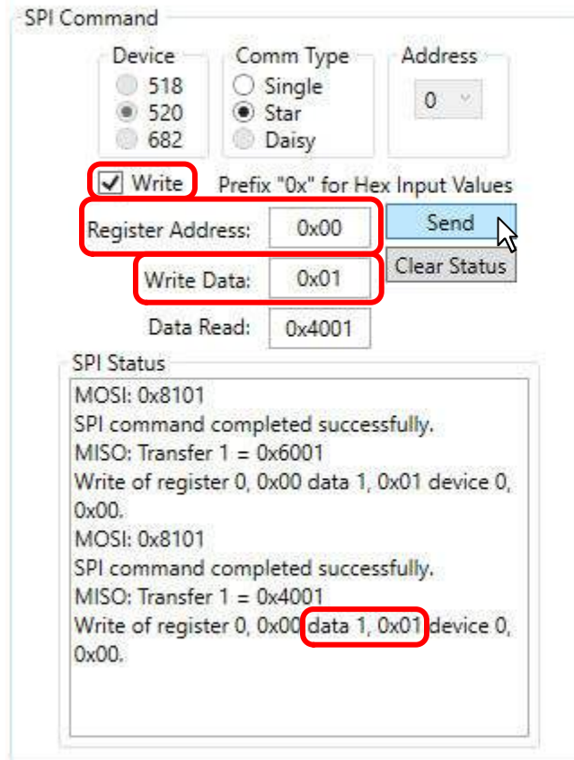
Figure 5-10. SPI Write Example
