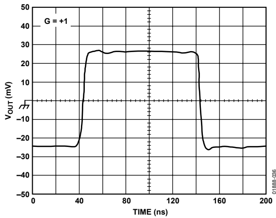
Figure 36. Small Signal Transient Response, V_O = 50 mV p-p, G = +1 (See Figure 48)
