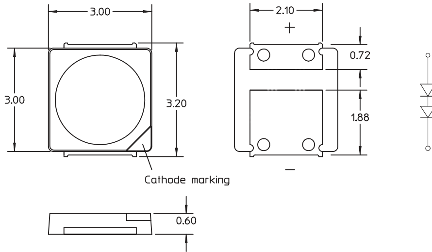
Figure 1 Package Dimensions
