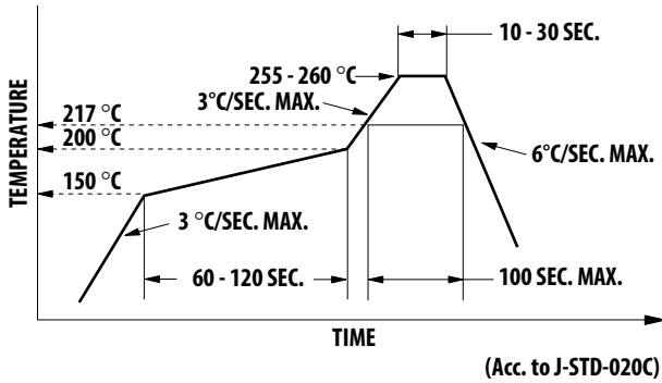
Figure 19 Reflow Soldering
