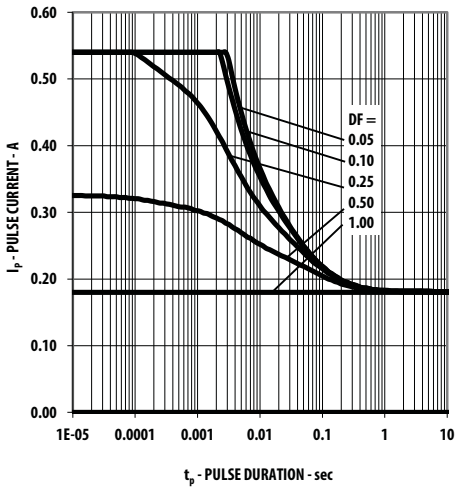
Figure 14 Pulse Handling Capability at T_C \leq 100^\circ\text{C}
