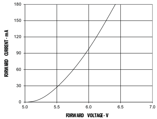
Figure 4 Forward Current vs. Forward Voltage
