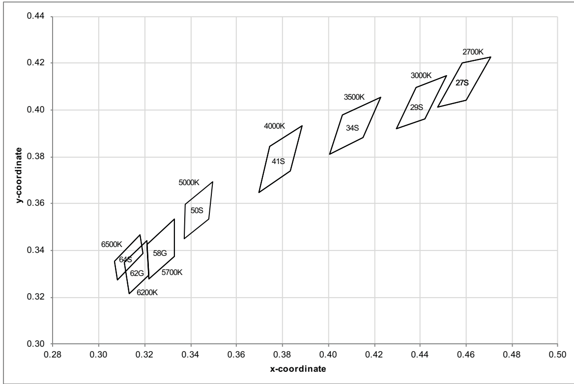
Figure 2 Chromaticity Diagram
