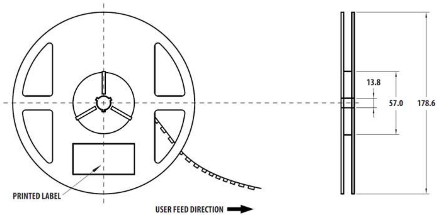
Figure 18 Reel Dimension
