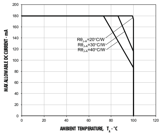
Figure 13 Derating Curve According to Ambient Temperature ( T_A )
