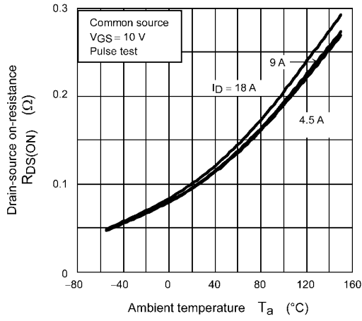
Fig. 8.7 R_{DS(ON)} - T_a
