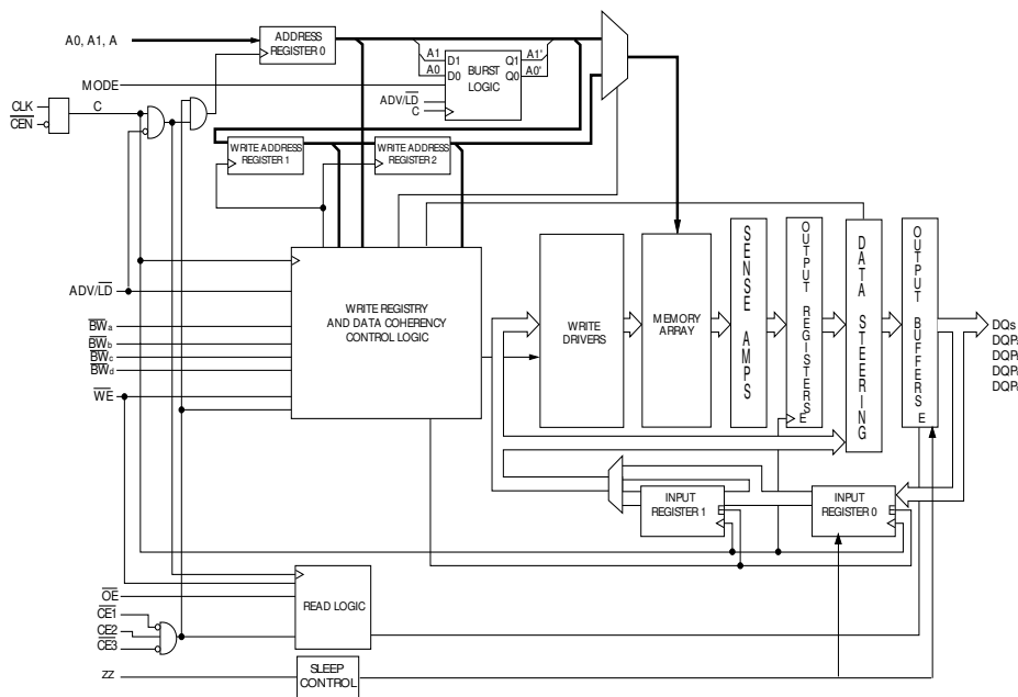
Logic Block Diagram—CY7C1354C (256K x 36)
