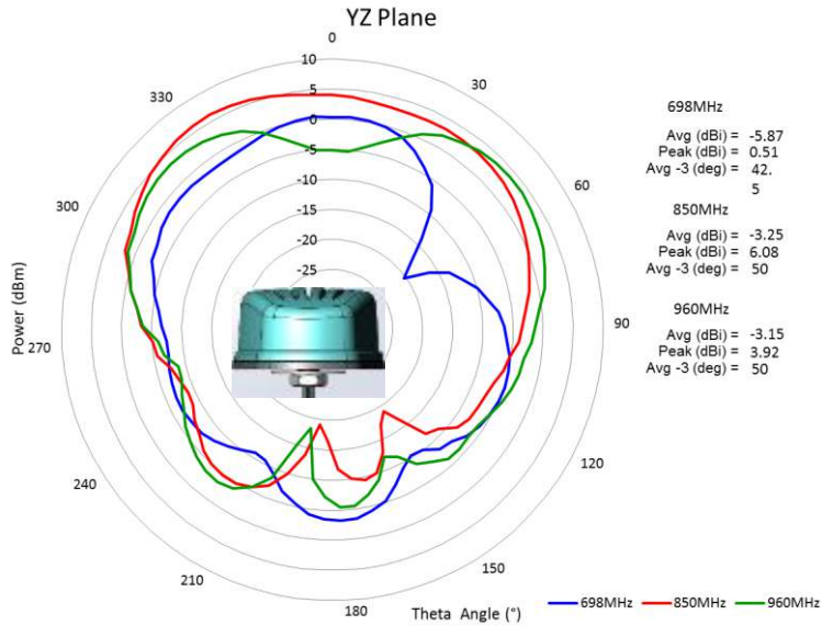
LTE1 antenna Y-Z plane radiation pattern at LTE low band**
