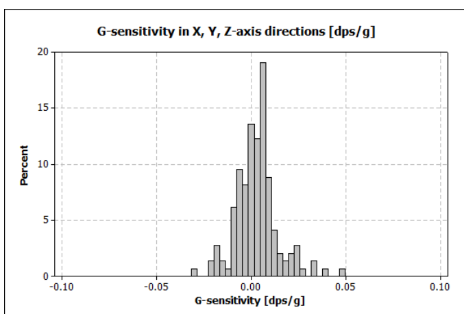
Figure 7. SCC2130-D08 gyro typical G-sensitivity in (°/s)/g.
