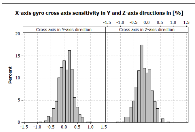
Figure 6. SCC2130-D08 gyro typical cross axis sensitivity in %.
