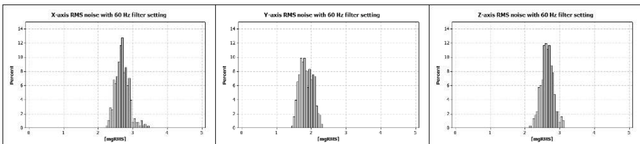
Figure 11. SCC2130-D08 accelerometer typical RMS noise in mg RMS .
