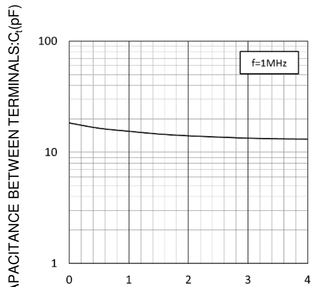
REVERSE VOLTAGE: V_R(V) V_R - C_t CHARACTERISTICS
