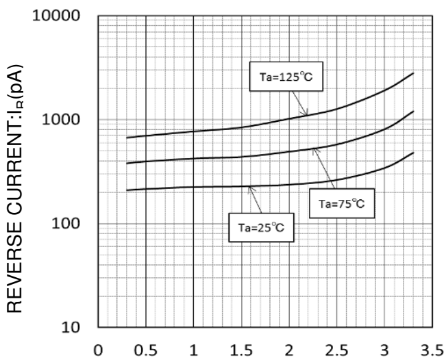
REVERSE VOLTAGE: V_R(V) V_R - I_R CHARACTERISTICS
