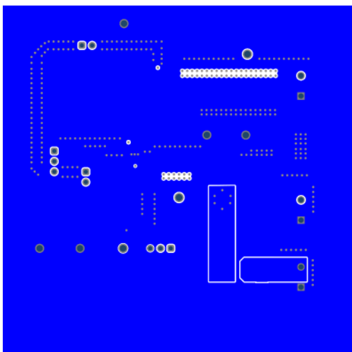
Figure 5-5. Bottom Layer
