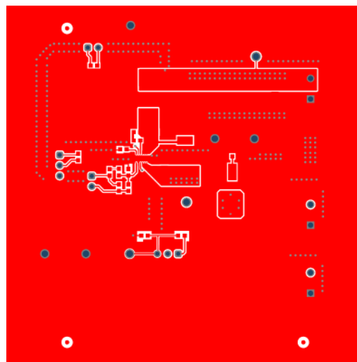
Figure 5-2. Top Layer
