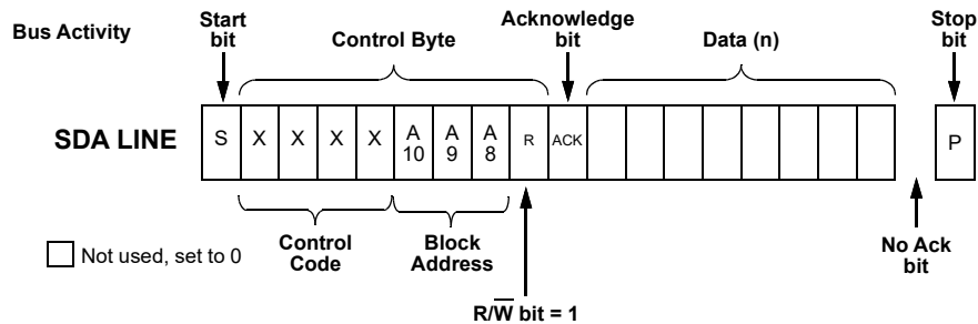
Figure 97: Current Address Read Command, R/\bar{W} = 1
