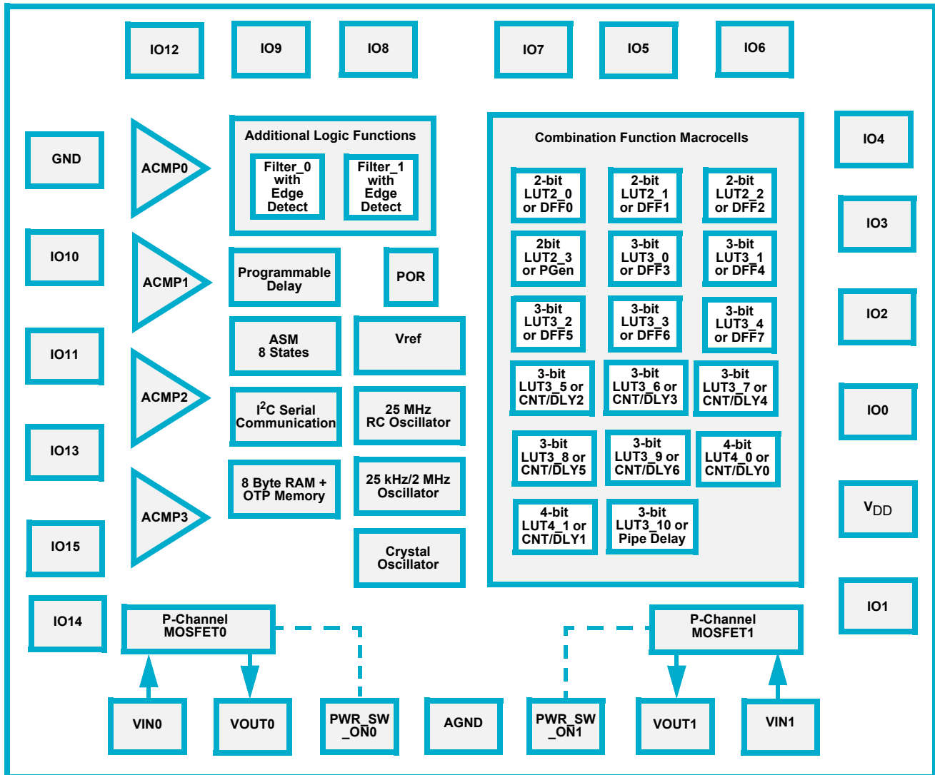
Figure 1: Block Diagram
