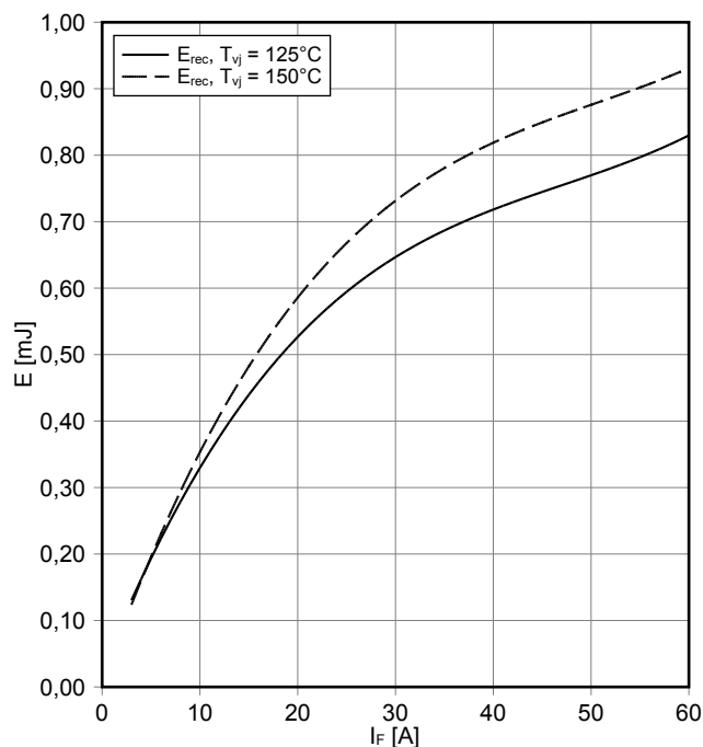
Schaltverluste Diode, D2 / D3 (typisch) switching losses Diode, D2 / D3 (typical) E_{rec} = f(I_F) R_{Gon} = 6.8 \Omega, V_{CE} = 400 V
