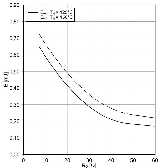
Schaltverluste Diode, D2 / D3 (typisch) switching losses Diode, D2 / D3 (typical) E_{rec} = f(R_G) I_F = 30 A, V_{CE} = 400 V
