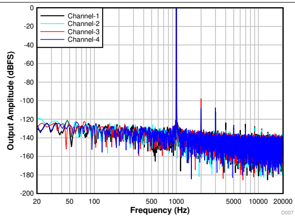
Figure 16. FFT With a -1-dBr Input
