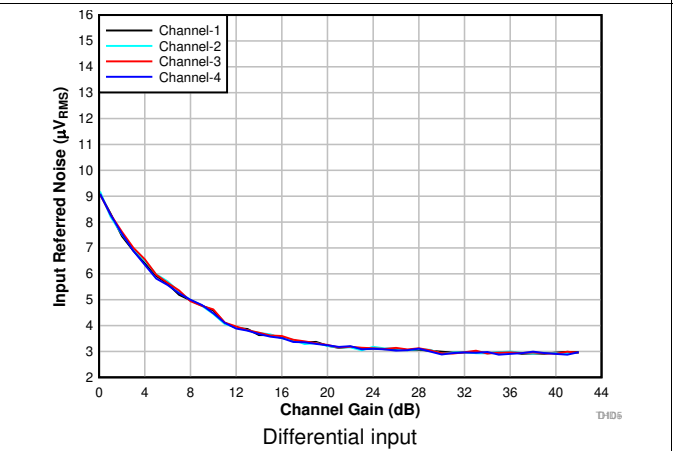
Figure 10. Input-Referred Noise vs Channel Gain
