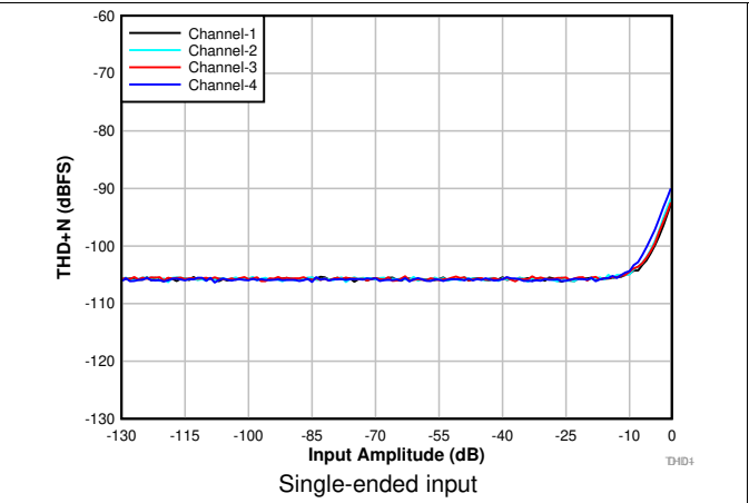
Figure 6. THD+N vs Input Amplitude
