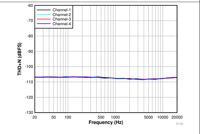
Figure 8. THD+N vs Input Frequency With a -60-dBr Input
