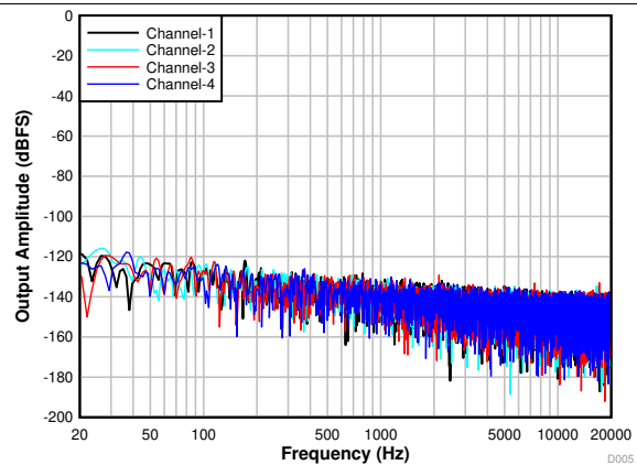
Figure 14. FFT With Idle Input
