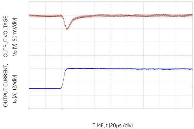
Figure 22. Transient Response to Dynamic Load Change from 50% to 100% at 12Vin, Cout = 4x47µF, CTune=2700pF & RTune=300Ω
