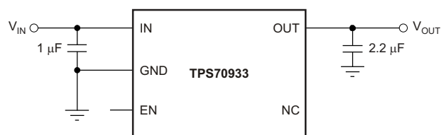
Figure 8-1. Wide Input, 3.3-V, Low- I_Q Rail
